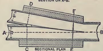
SECTIONAL PLAN E. FIG. 6. JUNCTION OF 8 FT. AND 11 FT. SEWERS.
